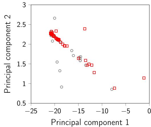
Figure 4-5: Features for sberbank projected on first two PCA components by FeatureHub (grey circles) and Deep Feature Synthesis (red squares).
